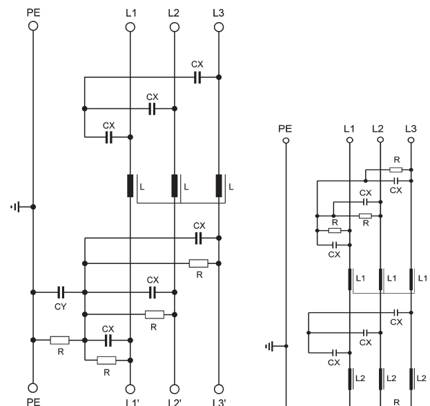
Fig. 7: Electrical diagram of Enerdoor single stage filter type FIN538
