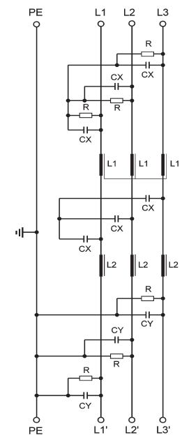
Fig. 8: Electrical diagram of Enerdoor double stage filter type FIN1500
